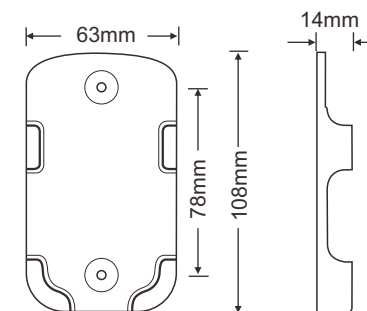
Remote holder
