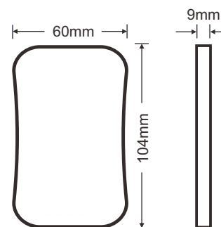
RF remote
