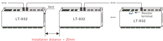
RJ45 connected in parallel
