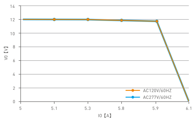
Over Load Diagram
