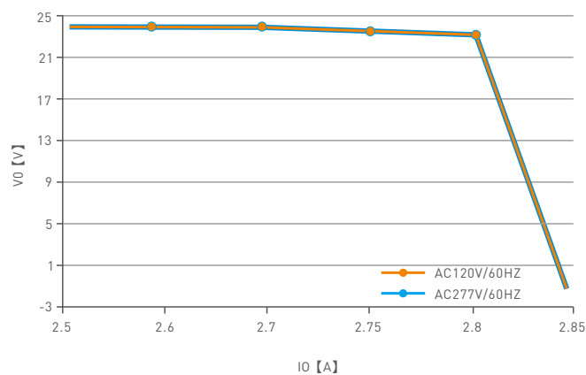
Over Load Diagram
